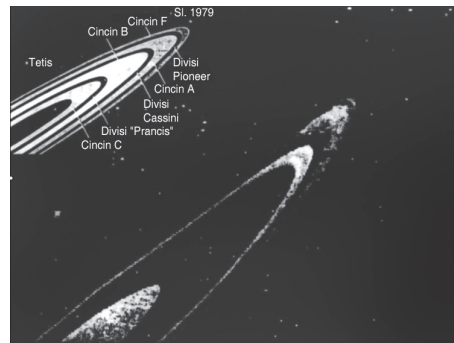
Gambar 2.16 Cincin-cincin Saturnus
