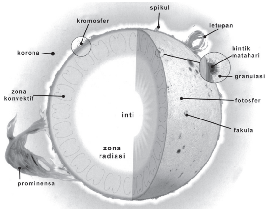
Gambar 2.6 Bagian-bagian matahari
