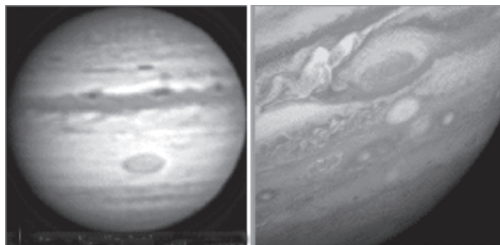
Gambar 2.14 Jupiter
